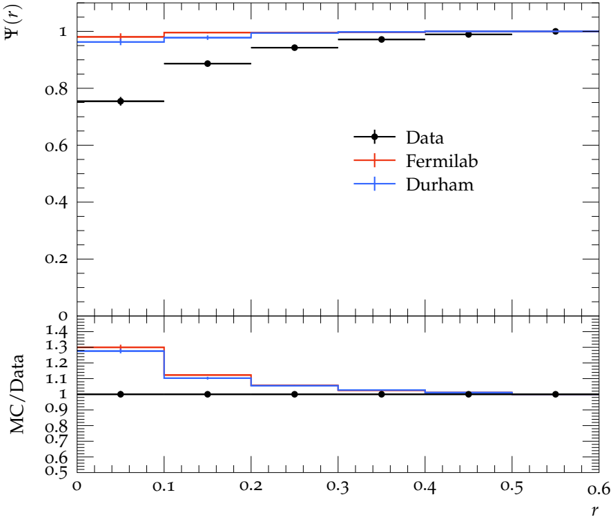
Jet shape \Psi for p_{\perp} \in 260\text{--}310\text{ GeV} , y \in 1.2\text{--}2.1
