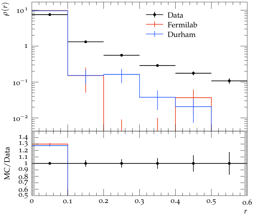
Jet shape \rho for p_{\perp} \in 260\text{--}310 GeV, y \in 1.2\text{--}2.1
