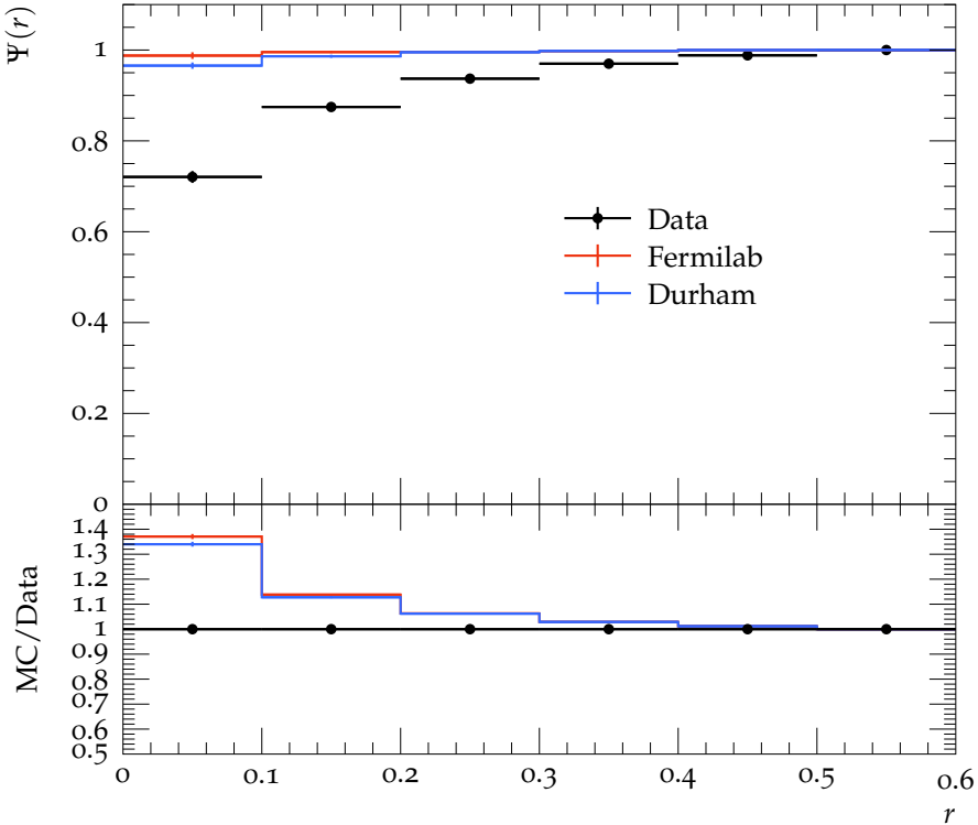
Jet shape \Psi for p_{\perp} \in 260\text{--}310\text{ GeV} , y \in 0.3\text{--}0.8
