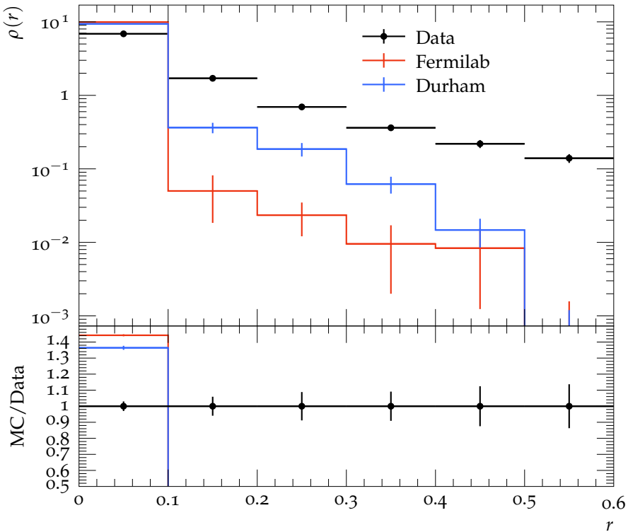
Jet shape \rho for p_{\perp} \in 210\text{--}260 GeV, y \in 0.3\text{--}0.8
