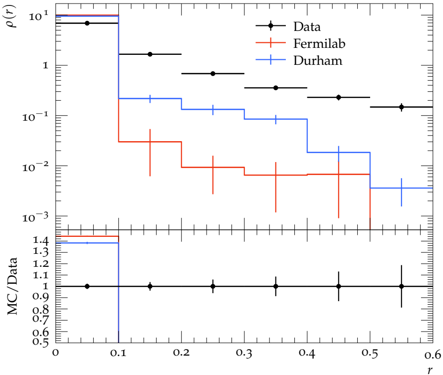
Jet shape \rho for p_{\perp} \in 160\text{--}210 GeV, y \in 1.2\text{--}2.1
