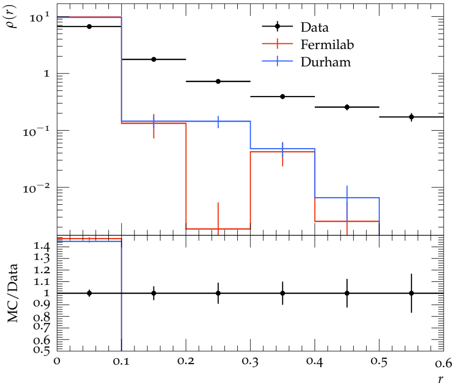
Jet shape \rho for p_{\perp} \in 110\text{--}160\text{ GeV} , y \in 2.1\text{--}2.8
