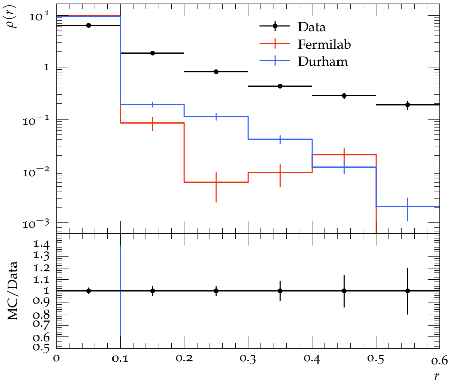
Jet shape \rho for p_{\perp} \in 110\text{--}160\text{ GeV} , y \in 1.2\text{--}2.1
