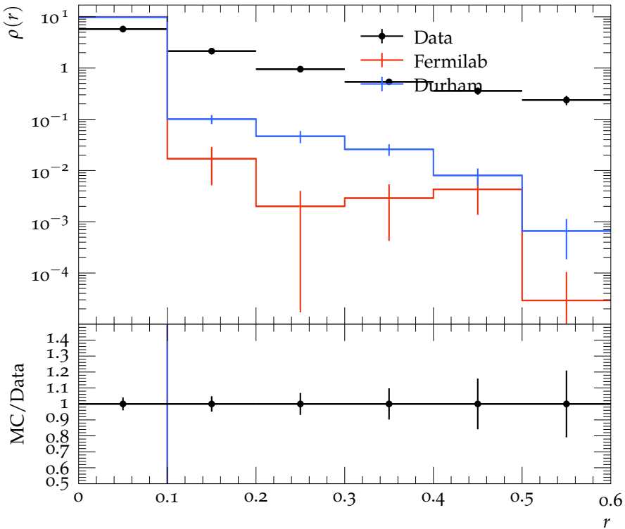
Jet shape \rho for p_{\perp} \in 80\text{--}110\text{ GeV} , y \in 1.2\text{--}2.1
