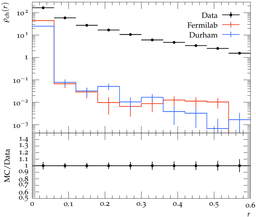
Density of charged particles for 80 \text{ GeV} < p_{T \text{ jet}} < 110 \text{ GeV}
