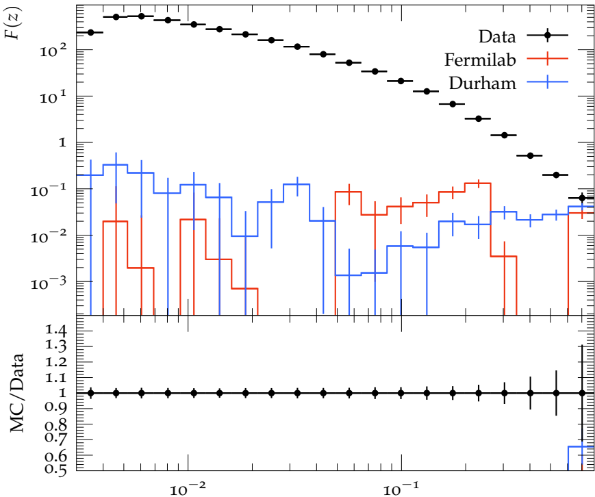
F(z) for 110 \text{ GeV} < p_{T \text{ jet}} < 160 \text{ GeV}
