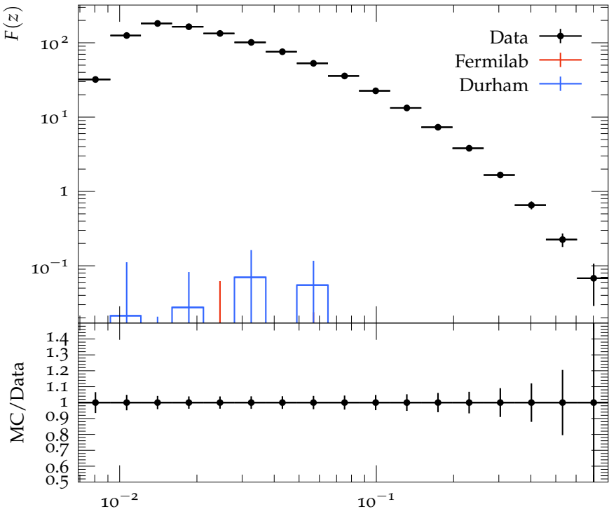
F(z) for 40 \text{ GeV} < p_{T \text{ jet}} < 60 \text{ GeV}
