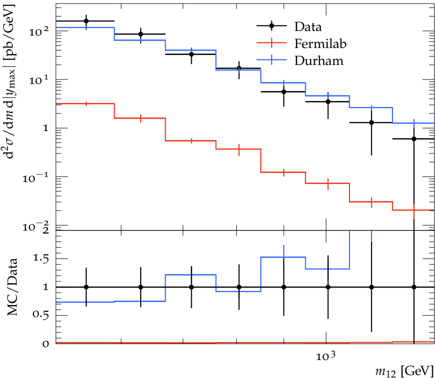
Dijet mass spectrum for 1.2 < |y_{\max}| < 2.1 . anti-KT, R = 0.6 .
