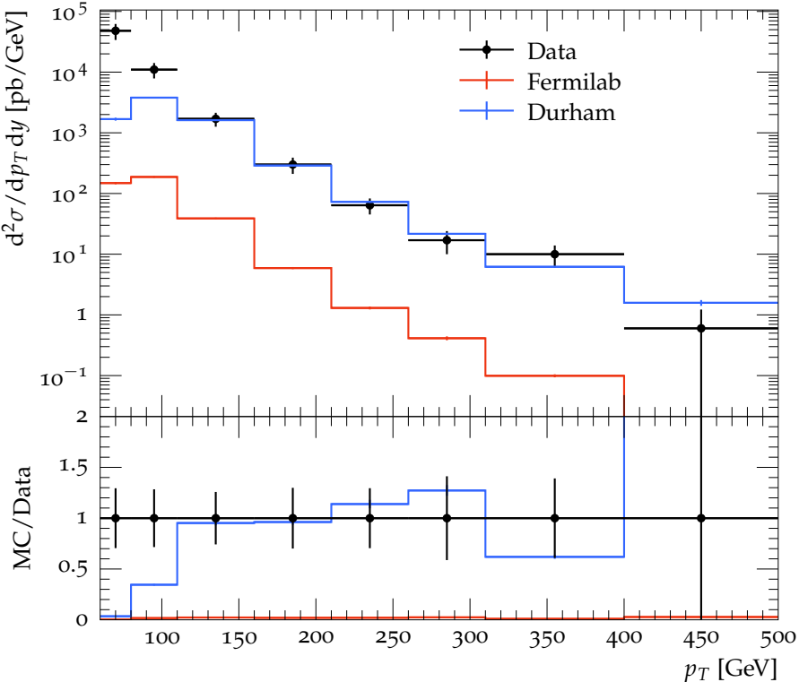
Inclusive jet p_T spectrum for 0.3 < |y| < 0.8 . anti-KT, R = 0.6 .
