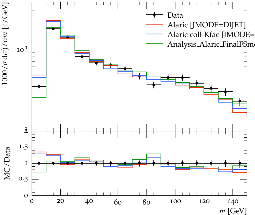
Pruned AK7 dijets, (p_T^1 + p_T^2)/2 = 800\text{--}1000 GeV
