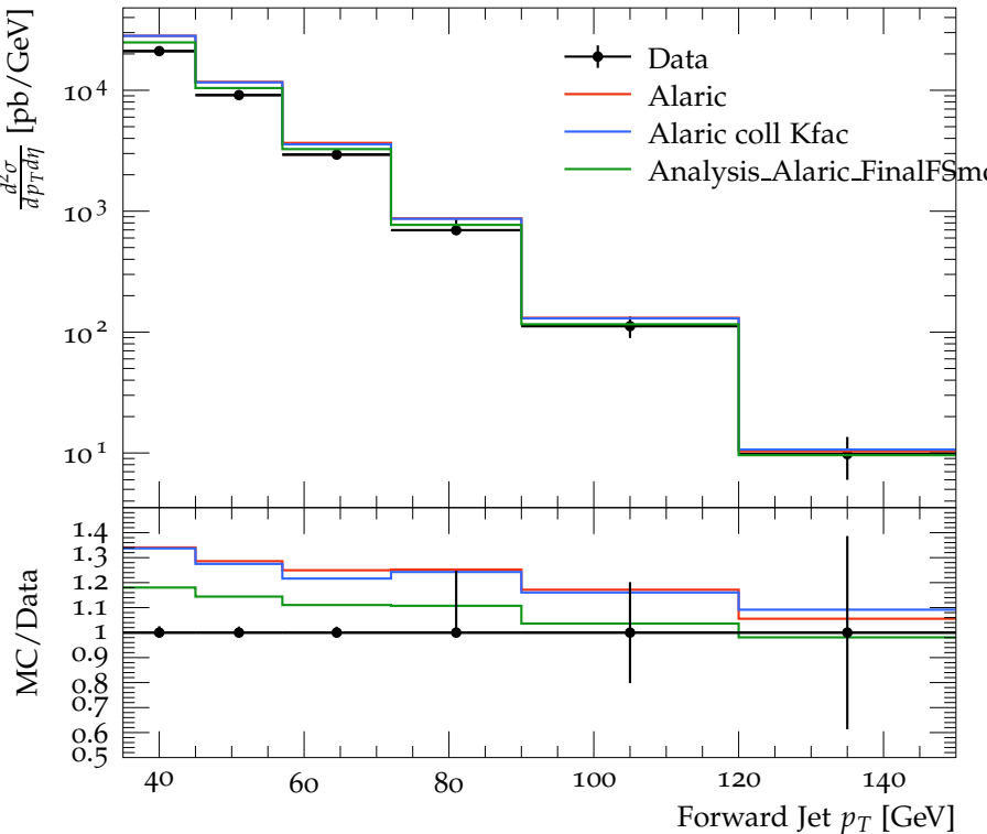
Measurement of forward+central jets at \sqrt{s} = 7 TeV
