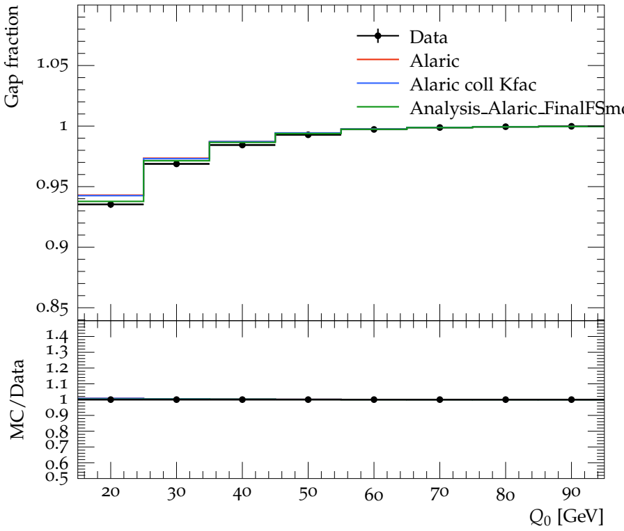
Gap fraction as a function of Q_0 for events satisfying 0 < \Delta y \leq 1
