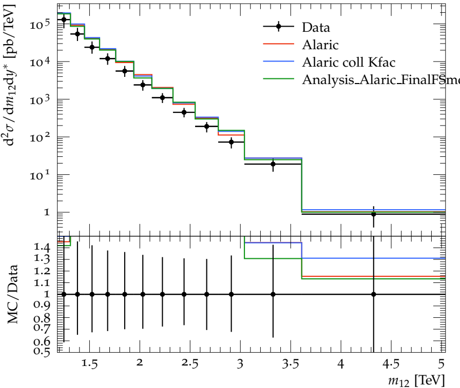
Dijet double-diff. x-section, anti- k_t 0.6 ( 3.0 \leq y^* < 3.5 )
