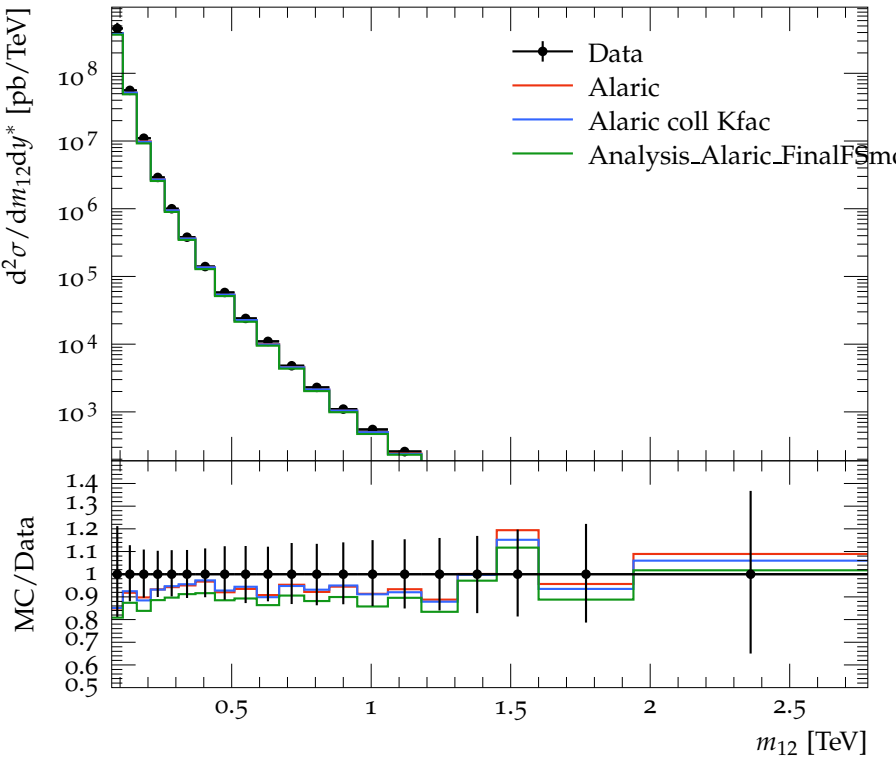
Dijet double-diff. x-section, anti- k_t 0.6 ( y^* < 0.5 )
