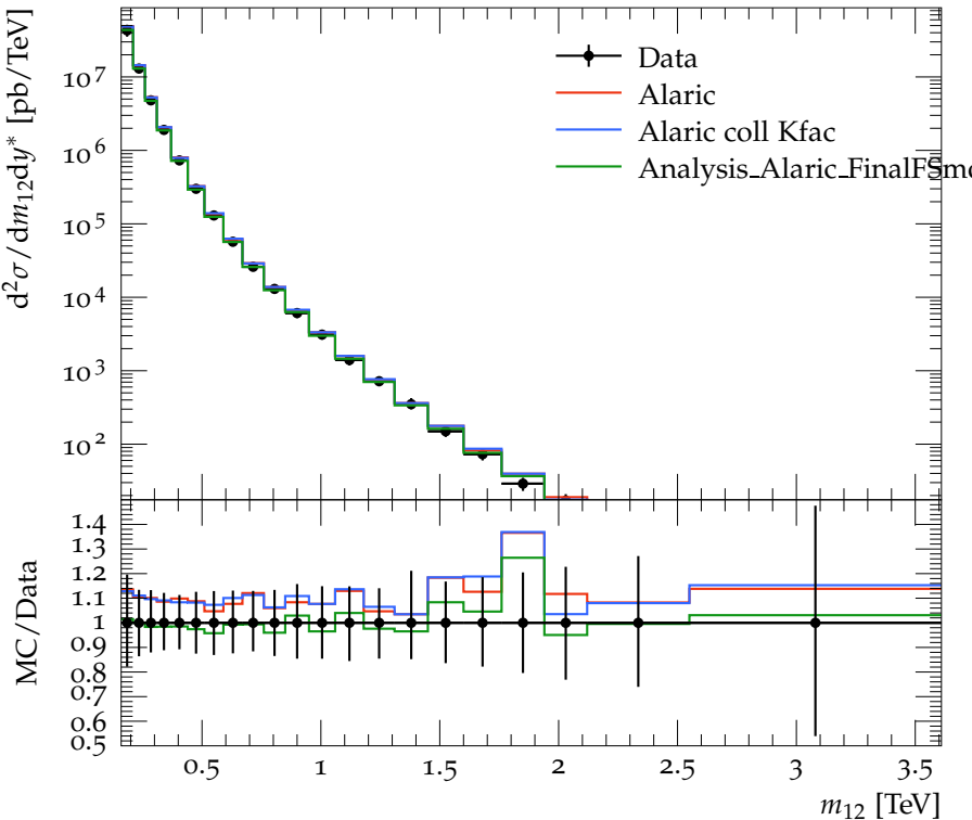
Dijet double-diff. x-section, anti- k_t 0.4 ( 1.0 \leq y^* < 1.5 )
