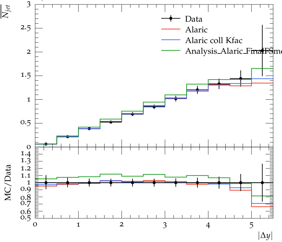
\overline{N}_{jet} vs |\Delta y| for 180 < \overline{P}_T < 210 , Leading Jet
