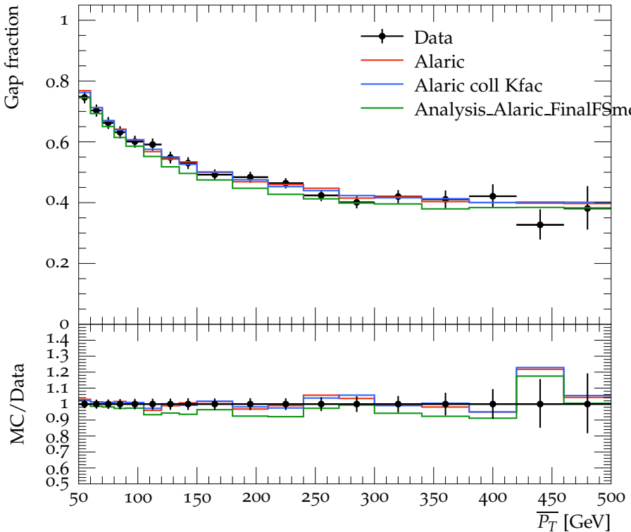
Gap fraction vs \overline{P_T} for 2.0 < |\Delta y| < 3.0 , Leading Jet
