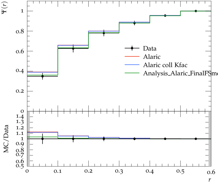
Jet shape \Psi for p_{\perp} \in 30\text{--}40\text{ GeV} , y \in 0.0\text{--}2.8
