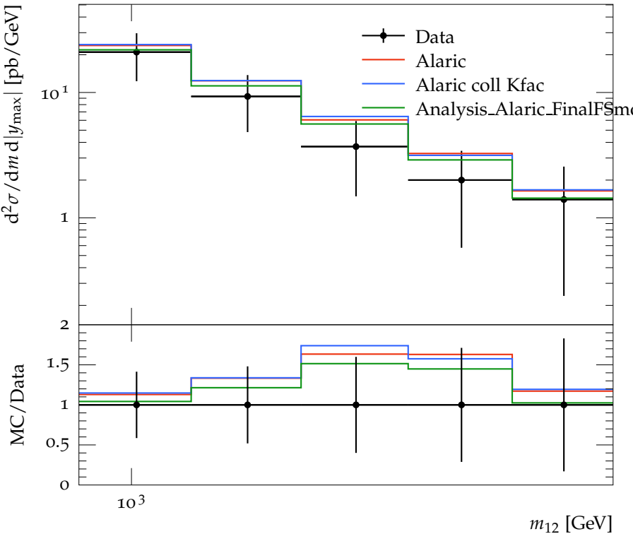
Dijet mass spectrum for 2.1 < |y_{\max}| < 2.8 . anti-KT, R = 0.4 .
