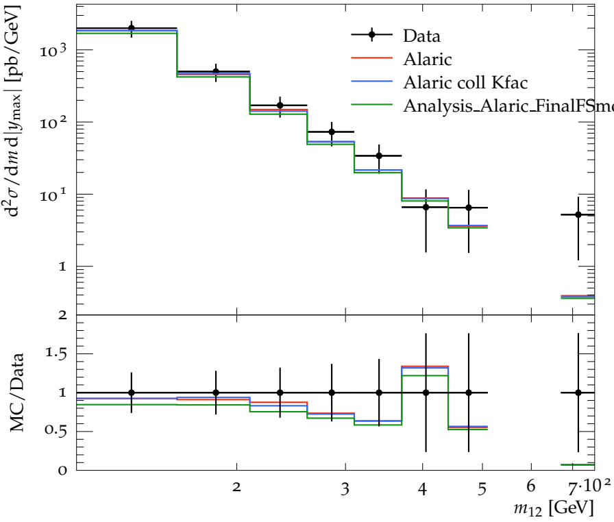
Dijet mass spectrum for |y_{\max}| < 0.3 , anti-KT, R = 0.4 .
