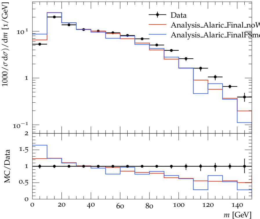
Pruned AK7 dijets, (p_T^1 + p_T^2)/2 = 450\text{--}500 GeV
