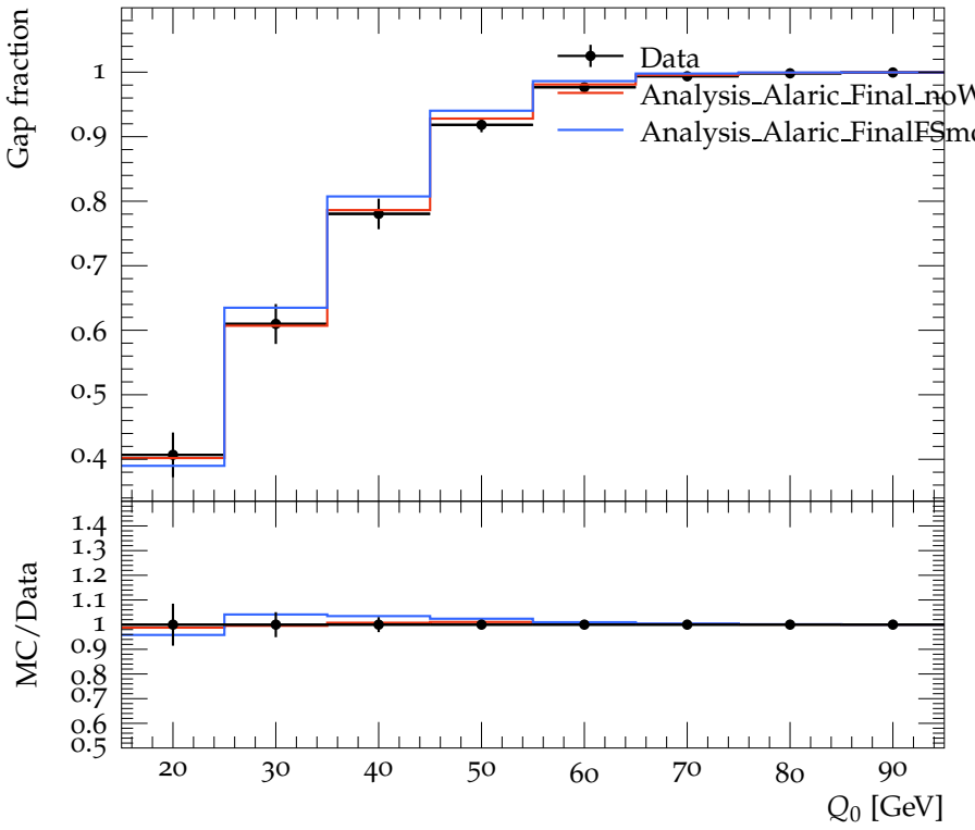
Gap fraction as a function of Q_0 for events satisfying 6 < \Delta y \leq 7
