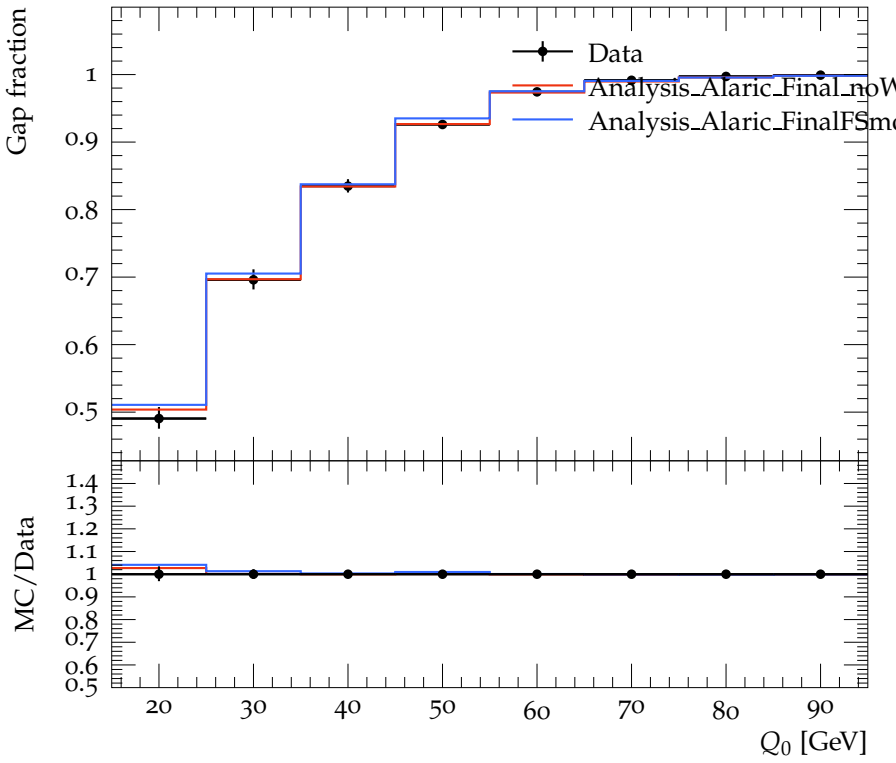
Gap fraction as a function of Q_0 for events satisfying 4 < \Delta y \leq 5
