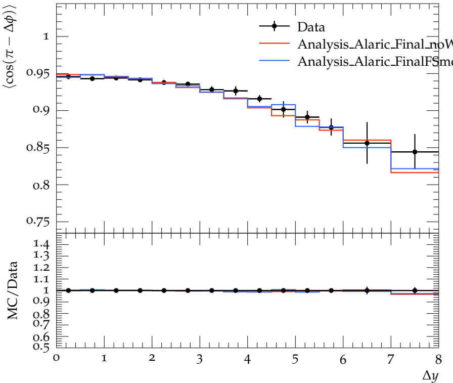
\langle \cos(\pi - \Delta\phi) \rangle for inclusive events as a function of \Delta y
