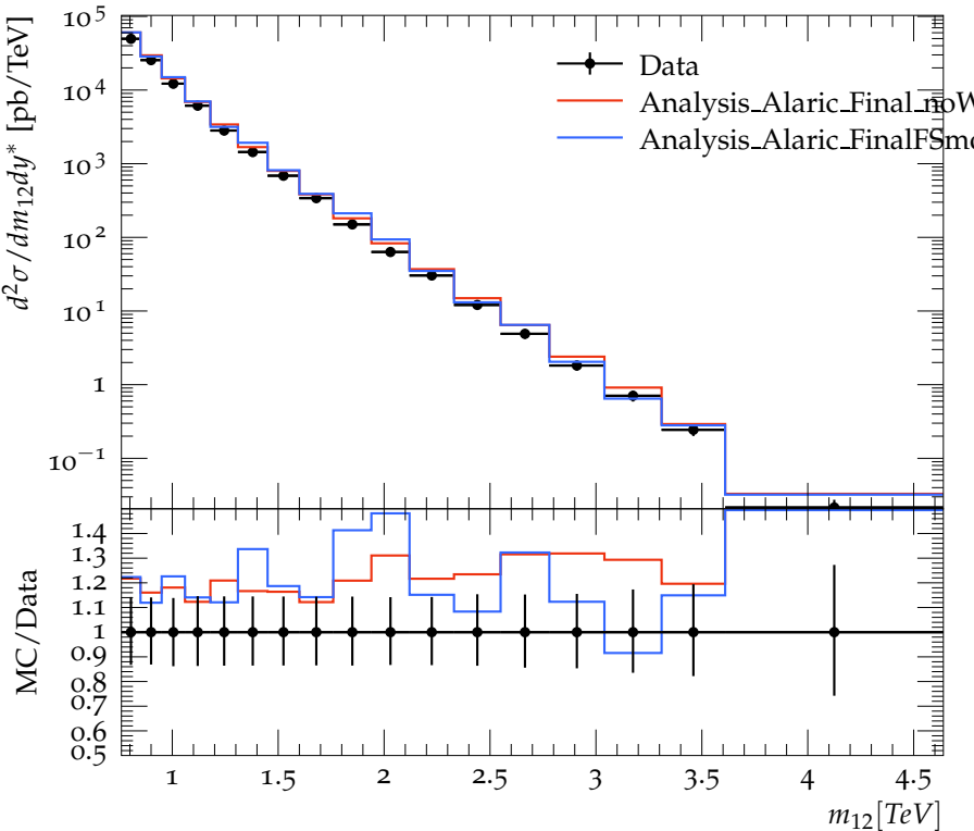
Dijet double-differential cross sections ( 1.5 < y^* < 2.0 ), R=0.6
