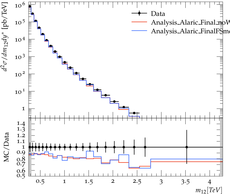
Dijet double-differential cross sections ( y^* < 0.5 ), R=0.4
