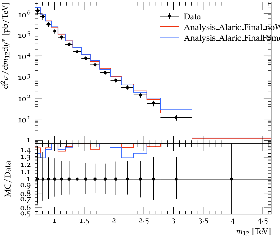
Dijet double-diff. x-section, anti- k_t 0.6 ( 2.5 \leq y^* < 3.0 )
