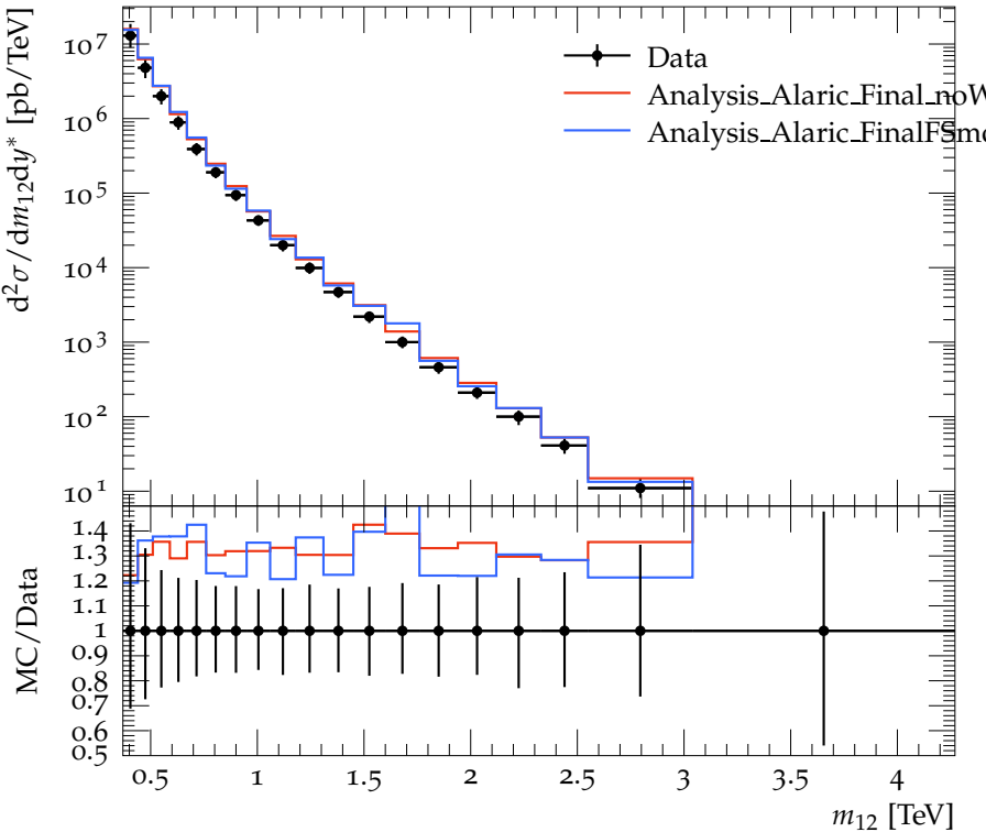
Dijet double-diff. x-section, anti- k_t 0.6 ( 2.0 \leq y^* < 2.5 )
