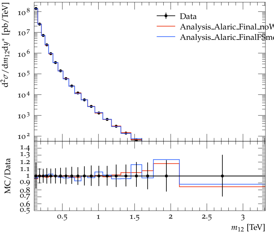
Dijet double-diff. x-section, anti- k_t 0.6 ( 0.5 \leq y^* < 1.0 )
