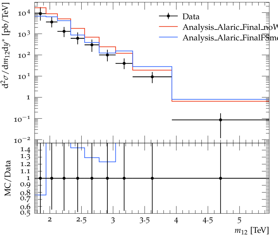
Dijet double-diff. x-section, anti- k_t 0.4 ( 3.5 \leq y^* < 4.0 )
