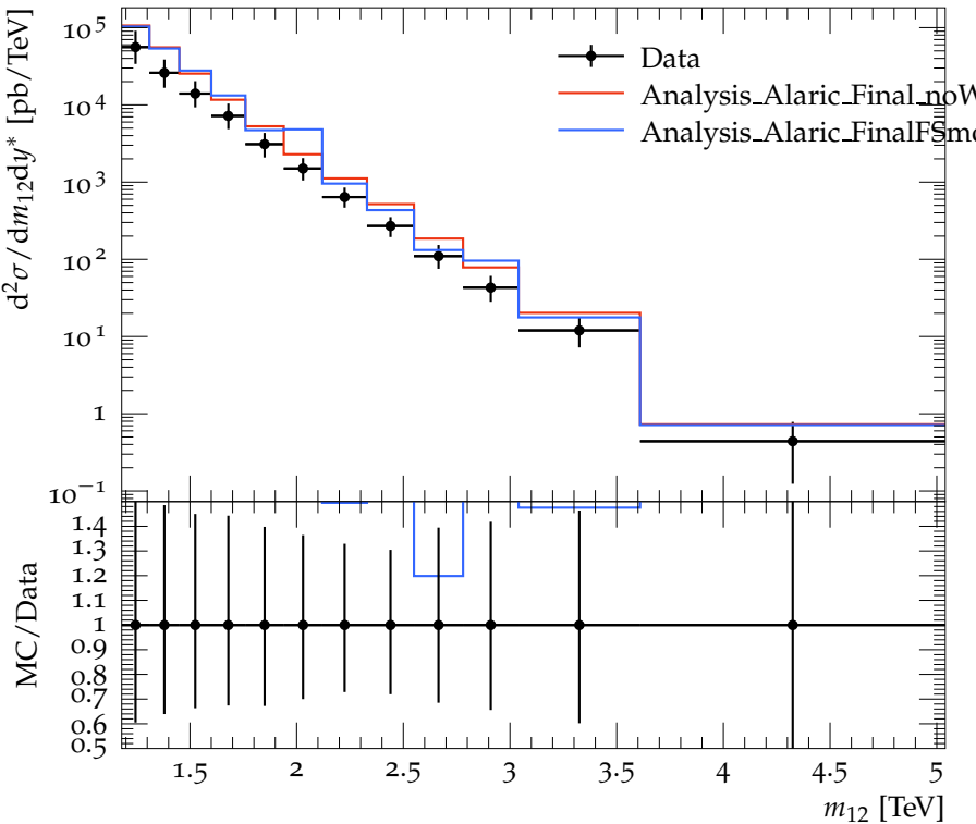
Dijet double-diff. x-section, anti- k_t 0.4 ( 3.0 \leq y^* < 3.5 )
