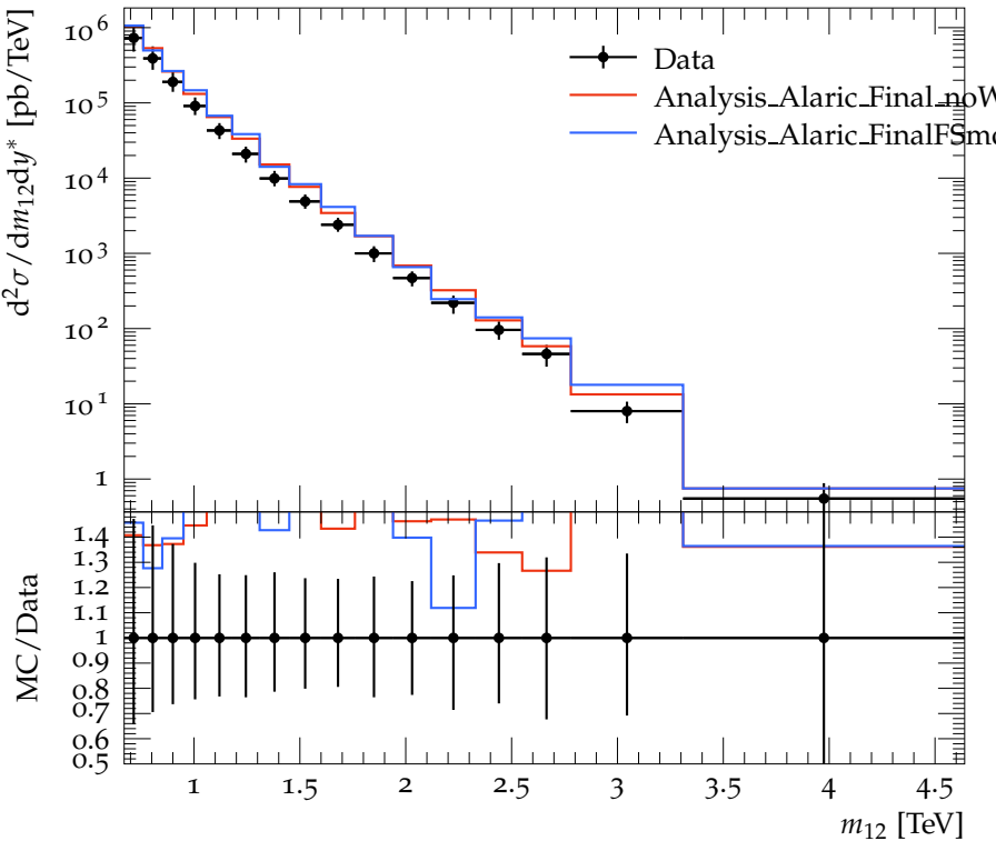
Dijet double-diff. x-section, anti- k_t 0.4 ( 2.5 \leq y^* < 3.0 )
