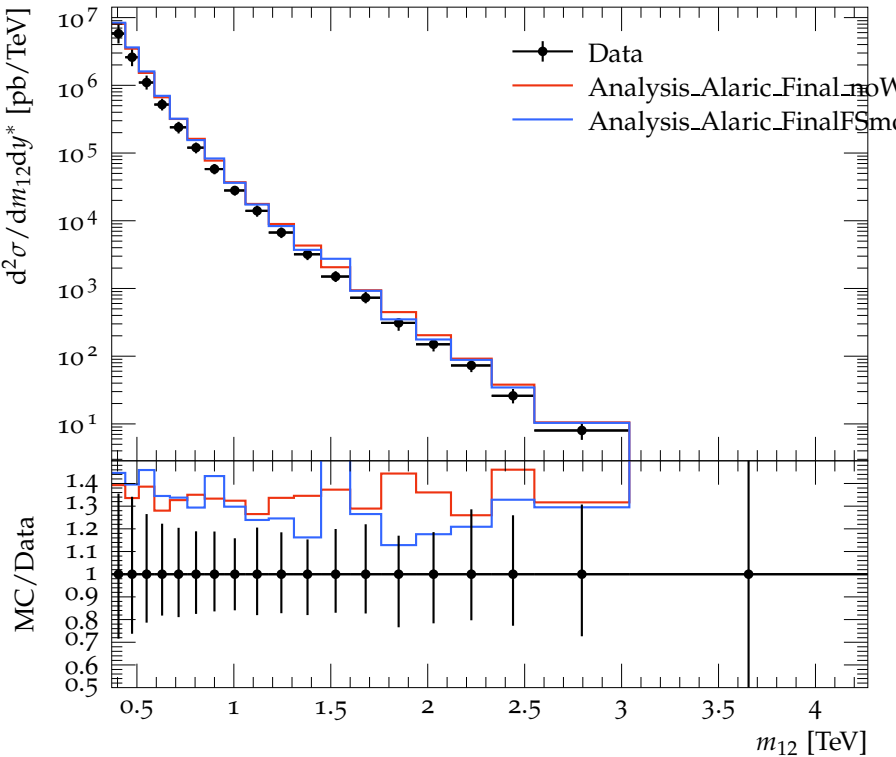
Dijet double-diff. x-section, anti- k_t 0.4 ( 2.0 \leq y^* < 2.5 )
