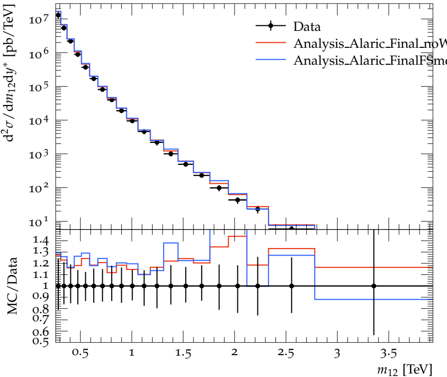
Dijet double-diff. x-section, anti- k_t 0.4 ( 1.5 \leq y^* < 2.0 )
