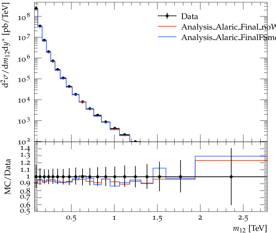
Dijet double-diff. x-section, anti- k_t 0.4 ( y^* < 0.5 )
