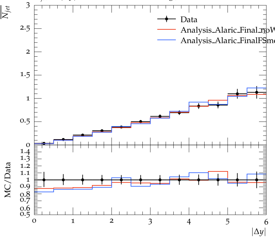
\overline{N}_{jet} vs |\Delta y| for 70 < \overline{P}_T < 90 , Leading Jet
