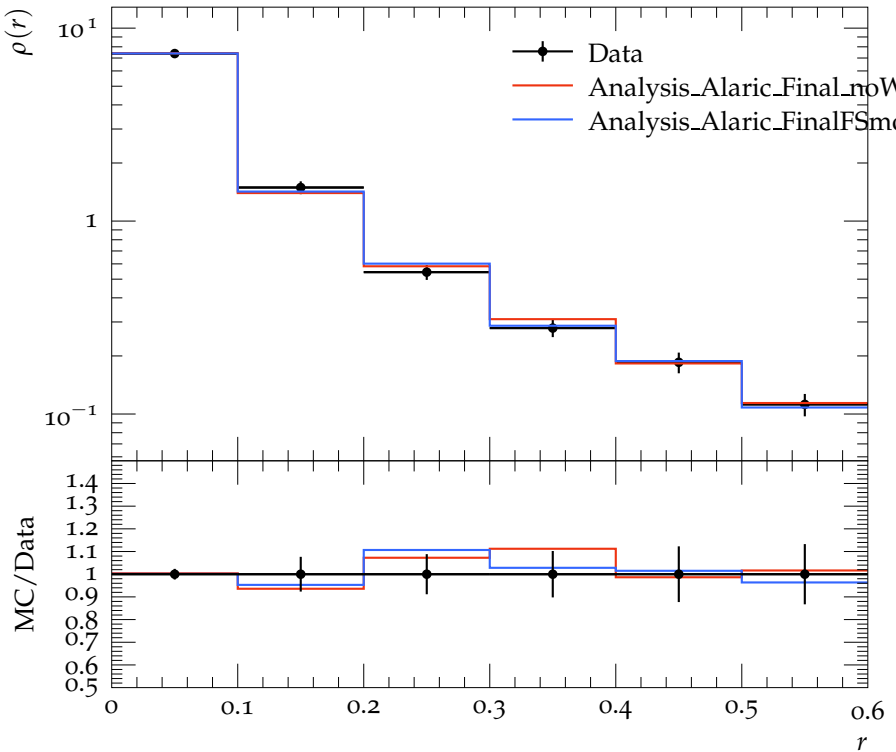
Jet shape \rho for p_{\perp} \in 310\text{--}400 GeV, y \in 0.0\text{--}0.3
