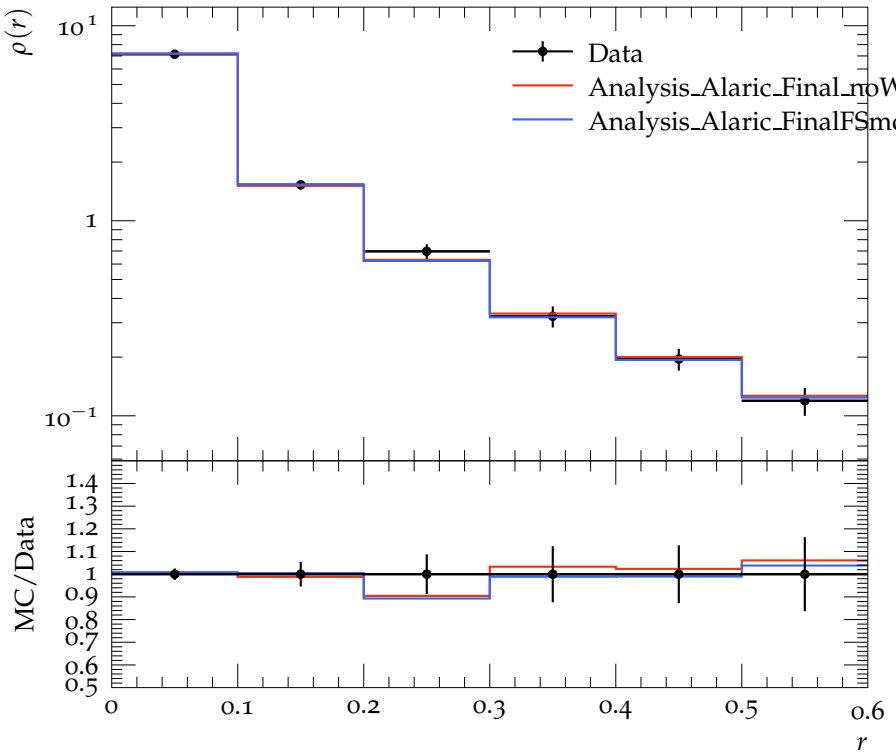
Jet shape \rho for p_{\perp} \in 260\text{--}310 GeV, y \in 0.0\text{--}0.3
