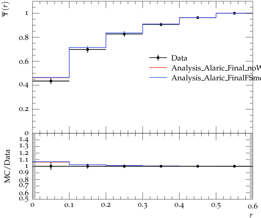
Jet shape \Psi for p_{\perp} \in 40\text{--}60\text{ GeV} , y \in 0.0\text{--}2.8
