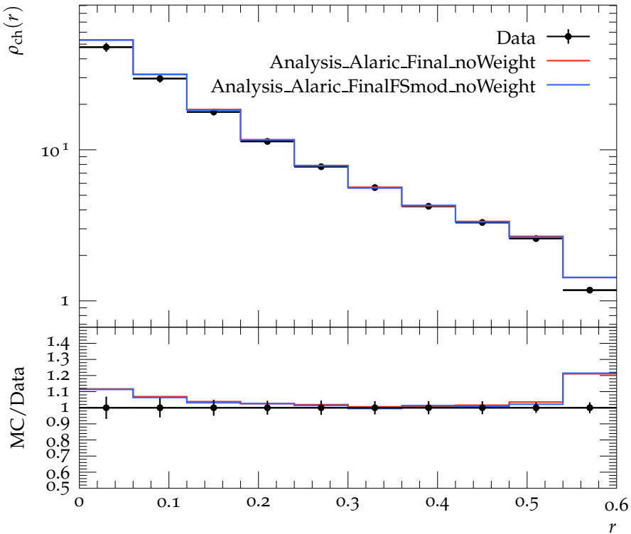
Density of charged particles for 25 \text{ GeV} < p_{T \text{ jet}} < 40 \text{ GeV}
