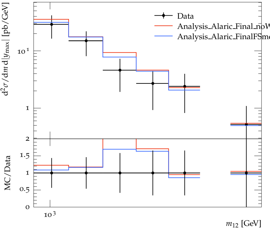
Dijet mass spectrum for 2.1 < |y_{\max}| < 2.8 . anti-KT, R = 0.6 .
