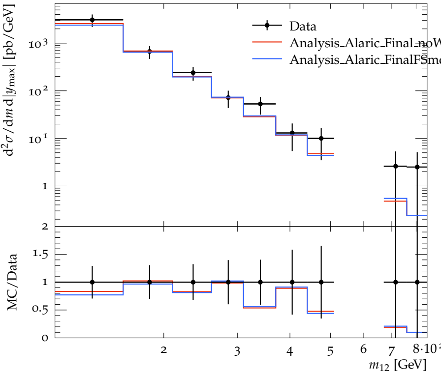
Dijet mass spectrum for |y_{\max}| < 0.3 . anti-KT, R = 0.6 .
