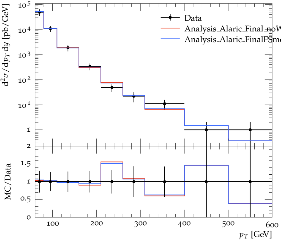
Inclusive jet p_T spectrum for |y| < 0.3 . anti-KT, R = 0.6 .
