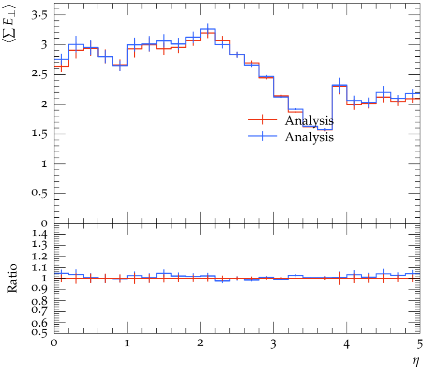
Pseudorapidity distribution of \langle \Sigma E_{\perp} \rangle
