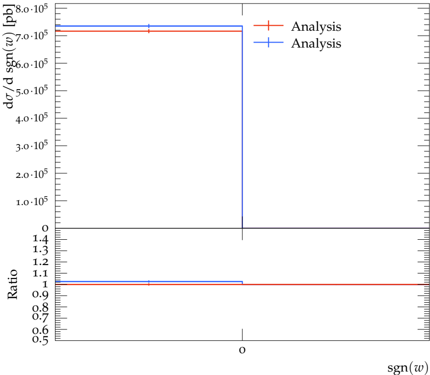
Fraction of events with positive and negative incoming lepton
