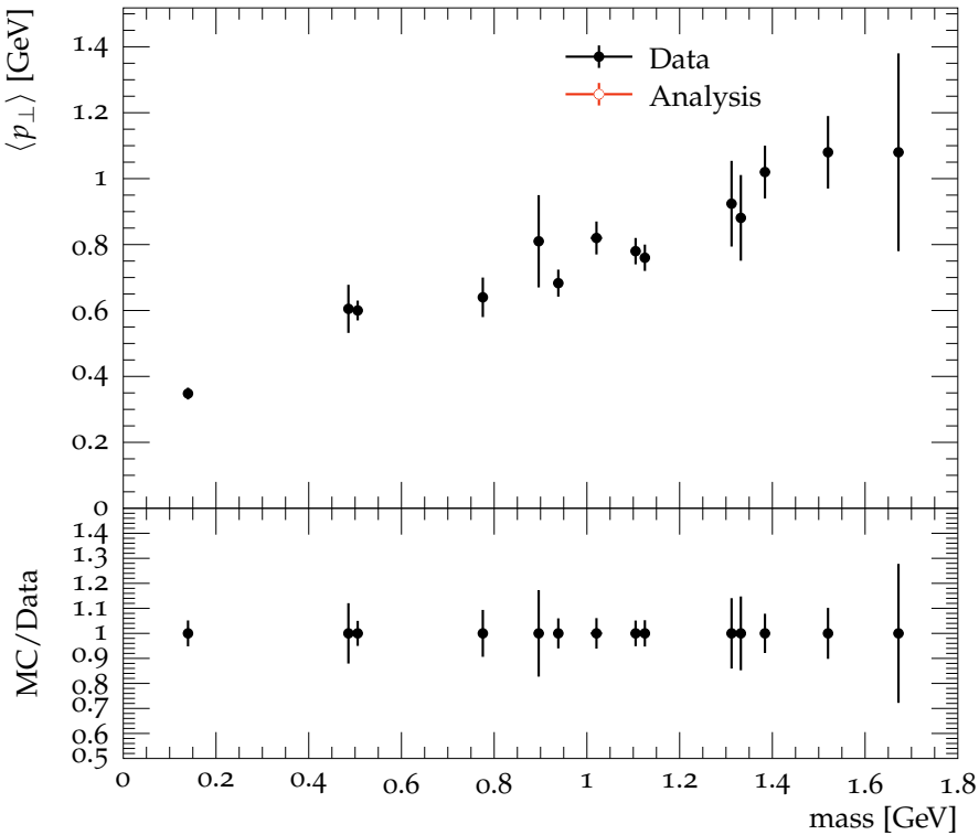
Mean p_{\perp} vs particle mass
